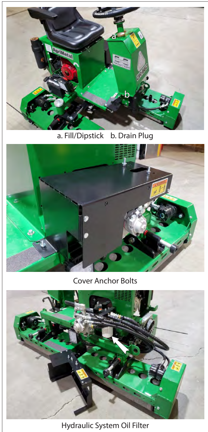
Fig. 55 HYDRAULIC SYSTEM
