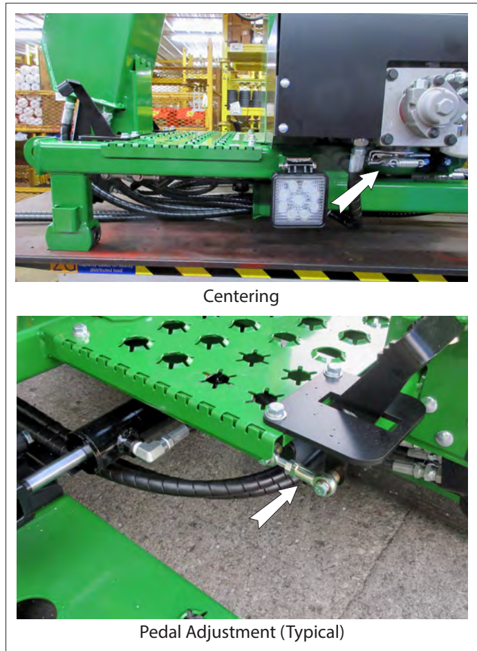
Fig. 56 ADJUSTING NEUTRAL
