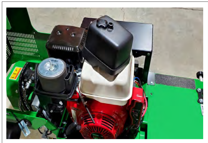
Fig. 53 AIR CLEANER
