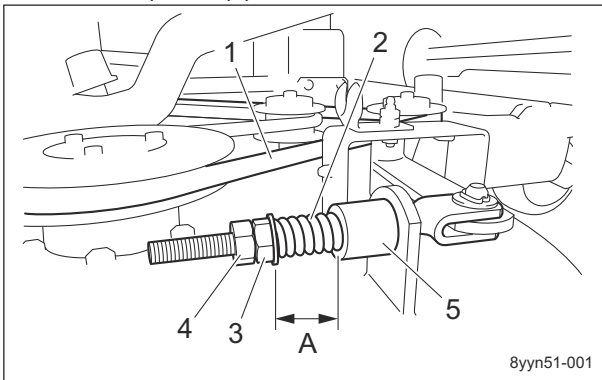
Adjustment of Left and Right Mower Deck Belts_001
