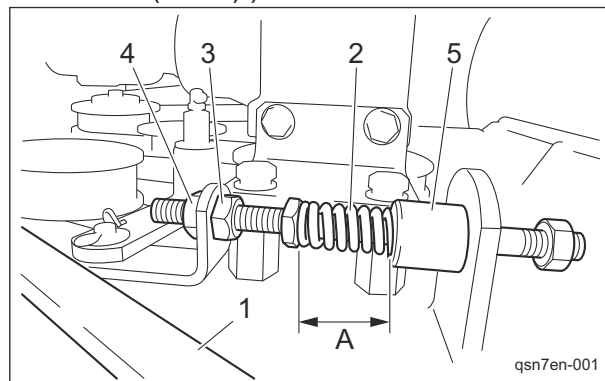
Adjustment of Center Mower Deck Belt_001
