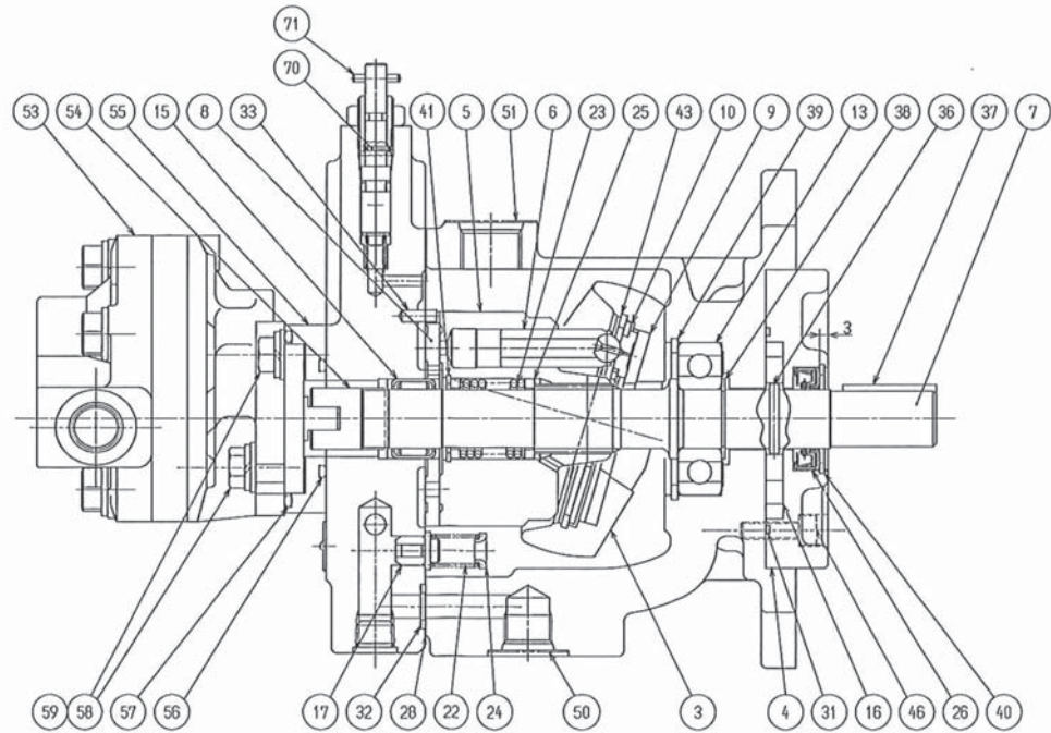
K3241000200 PUMP, PISTON PSV-16CHG-2
