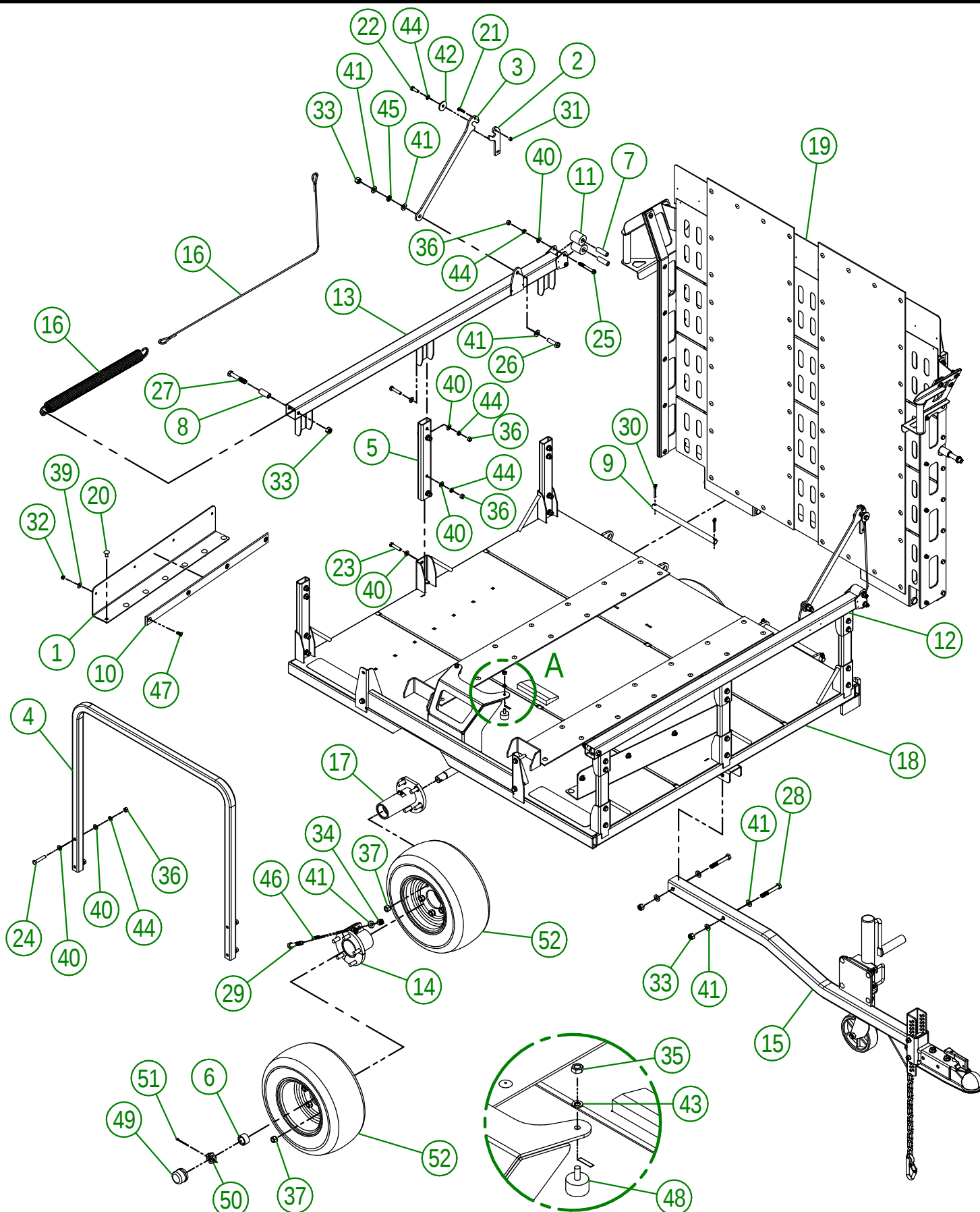
DETAIL A
