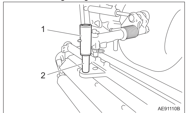
Installation of Verti Cutter (LS6 Installed Type)_002
