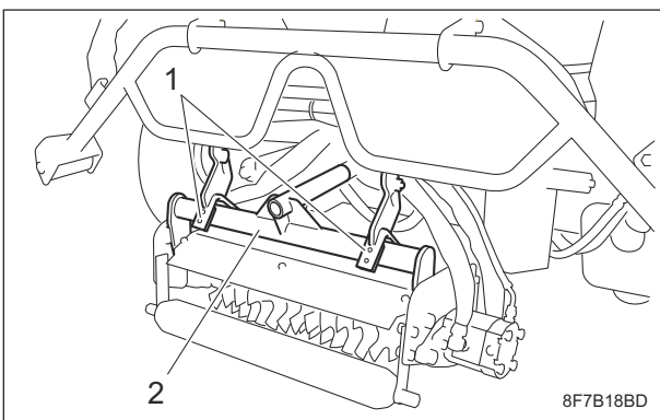
Installation of Verti Cutter (LH6 Installed Type)_006
