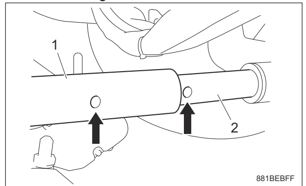
Installation of Verti Cutter (LH6 Installed Type)_003
