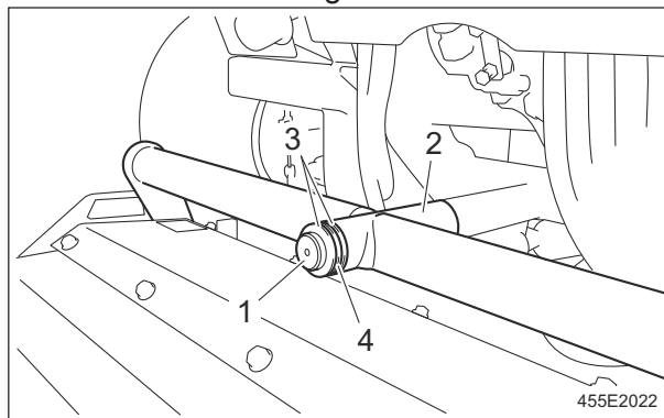
Installation of Verti Cutter #1 (LH6/LS6 Installed Type)_002
