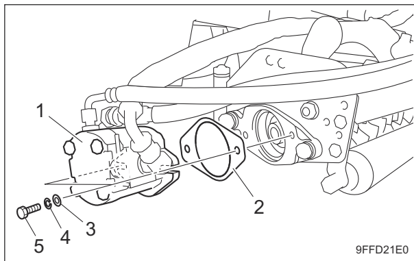
Installation of Verti Cutter #2·#3 (LS6 Installed Type)_003
