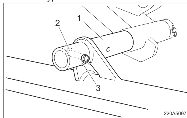
Removal of Verti Cutter_003
