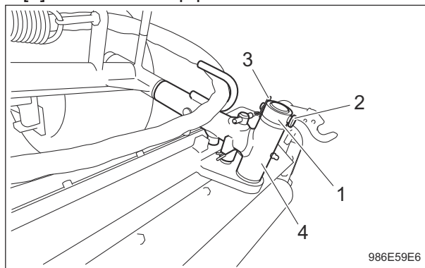
Installation of Verti Cutter #2·#3 (LS6 Installed Type)_002
