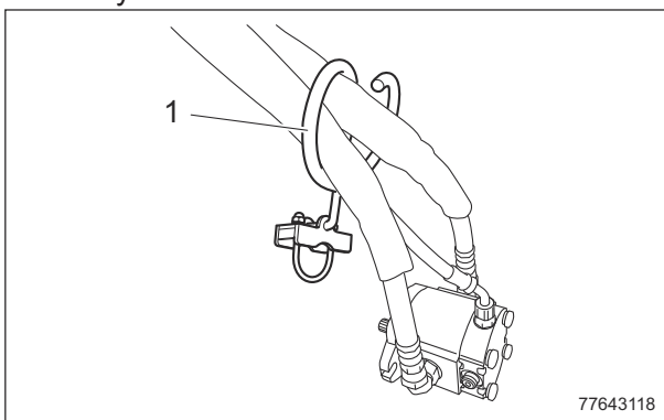
Installation of Verti Cutter (LS6 Installed Type)_001
