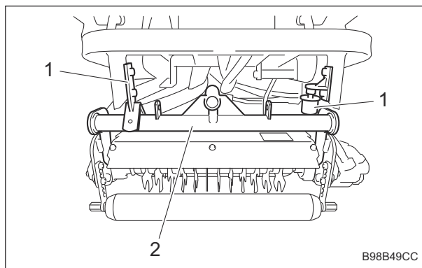
Installation of Verti Cutter_006
