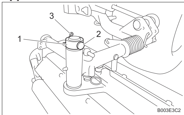
Removal of Verti Cutter (LS6 Installed Type)_002
