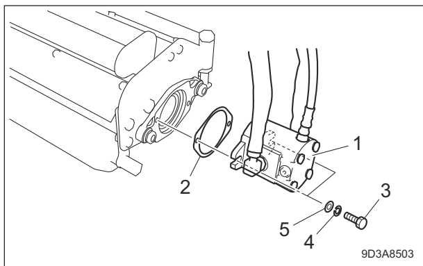
Installation of Verti Cutter_004
