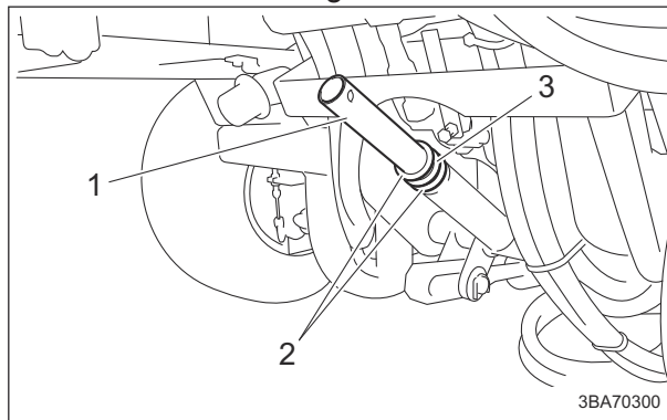
Installation of Verti Cutter #1 (LH6/LS6 Installed Type)_001
