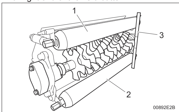
Adjustment of Cutting Depth_001
